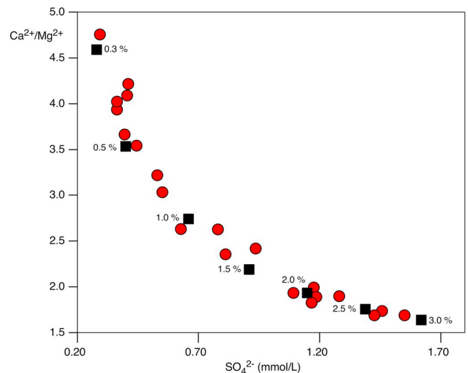
Fig. 7. Plot of Ca^{2+}/Mg^{2+} molar ratio as a function of SO_4^{2-} concentration in the MSA water (red circles). The black squares represent calculated values obtained for a two-component mixing, where a Ca-HCO_3 -type water ( Ca^{2+}/Mg^{2+} molar ratio = 7.1, SO_4^{2-} = 0.17 mmol/L and pH = 7.8) mixes with a sulfate-rich, thallium contaminated end member ( Ca^{2+}/Mg^{2+} molar ratio = 1.0, SO_4^{2-} = 32.3 mol/L and pH = 6.6) (see Section 5.1 for explanations). Numbers refer to the mixing percentage of SO_4^{2-} and Tl contaminated end member. (For interpretation of the references to color in this figure legend, the reader is referred to the web version of this article.)
