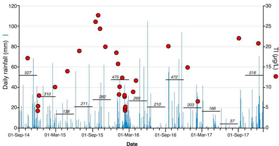
Fig. 3. Comparison between daily rainfall at the Pietrasanta raingauge ( www.sir.toscana.it ) and Tl concentrations in water from the MSA spring. The numbers in italics are the cumulative rainfall (mm) over the indicated time intervals (black horizontal segments).
