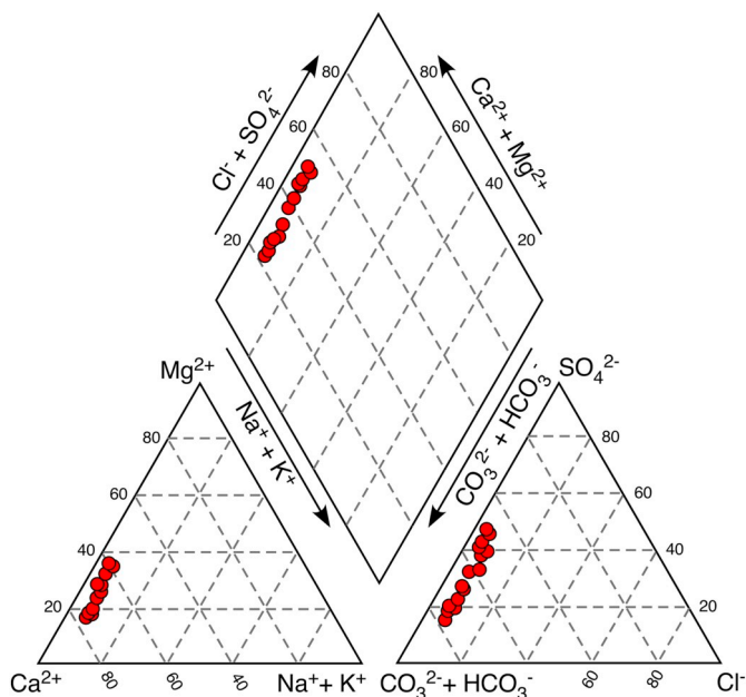
Fig. 2. Piper diagram for the MSA waters.
