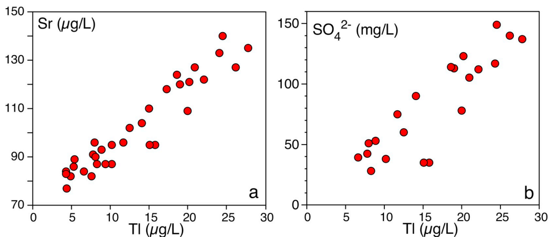
Fig. 5. Plot of Sr vs. Tl (a), and SO 4 2- vs. Tl (b) in the MSA spring water.
