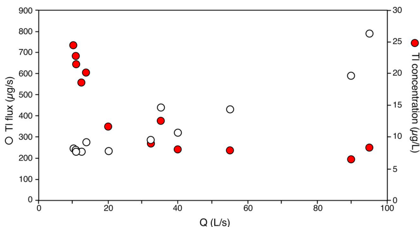
Fig. 4. Plot of Tl concentration (red circles) and Tl flux (empty circles) at MSA spring as a function of the spring flow rate (Q). (For interpretation of the references to color in this figure legend, the reader is referred to the web version of this article.)
