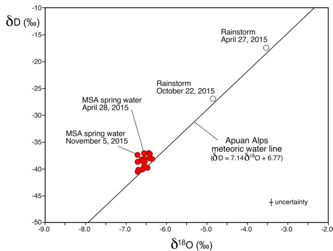
Fig. 6. Plot of \delta D (‰) vs. \delta^{18}O (‰) for water samples from the Molini di Sant'Anna spring. The rainwater of rainstorm events of April 27 and October 22, 2015 are also plotted. The Apuan Alps meteoric water line determined by Mussi et al. (1998) is drawn for comparison.
