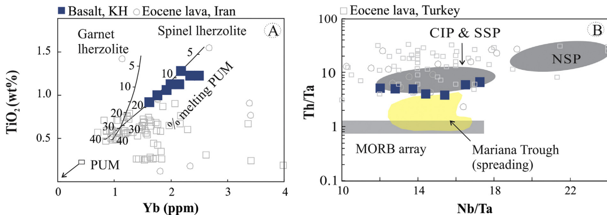
Fig. 9. Plots to estimate the degrees of partial melting that generated the Kahrizak basalts. (A) \text{Ti} versus \text{Yb} with a fixed primitive upper mantle (PUM) composition (Gribble et al., 1996). This plot assumes that the Mariana Trough backarc basin basalts (BABB) were produced by 6% to 24% partial melting in the spinel lherzolite stability field, with the highest value of 34% representing an arc-like basalt (Pearce and Stern, 2006). (B) \text{Th}/\text{Ta} (a proxy for the deep subduction component) versus \text{Nb}/\text{Ta} (a proxy for degree of melting and mantle depletion). Central and southern Mariana arcs = CIP and SSP, respectively and northern Mariana arc = NSP. See text for discussion.
