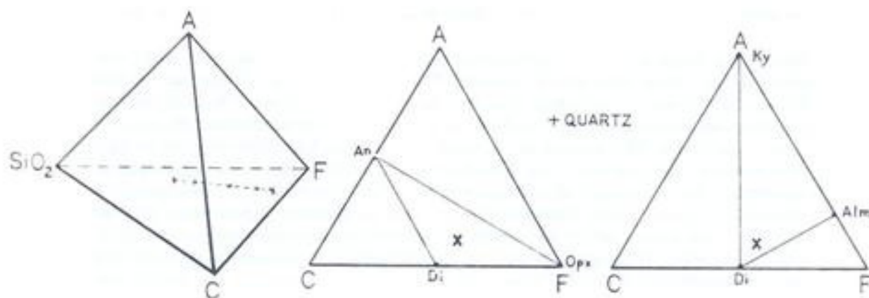
Figure 6-1 ACF diagram for rocks containing quartz. Rock compositions are projected from \text{SiO}_2 onto the ACF face of the tetrahedron (see text for explanation). Under one set of metamorphic conditions a rock with bulk composition X might consist of the mineral assemblage quartz-anorthite-diopside-orthopyroxene, but under another set of conditions would consist of quartz-kyanite-diopside-almandine.
