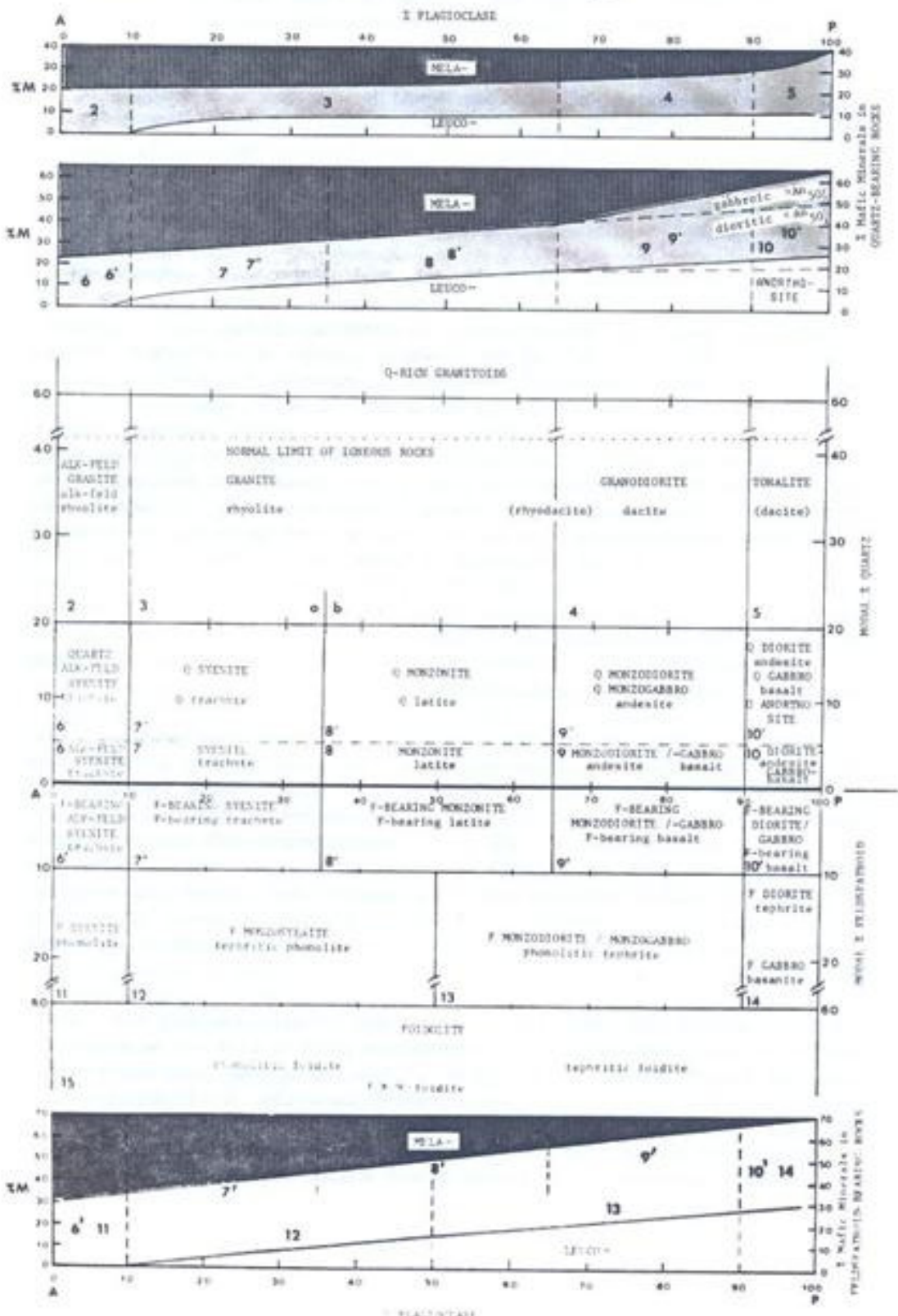
Figure 4-1 IUGS classification of igneous rocks containing less than 90% mafic minerals. Plutonic rocks are in upper case and volcanic ones in lower case letters. A = alkali feldspar + albite (<math>A_{Al_5}</math>) and P = plagioclase (>math>A_{An_5}</math>).
