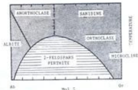
Schematic representation of relative temperatures at which various alkali feldspars form.
