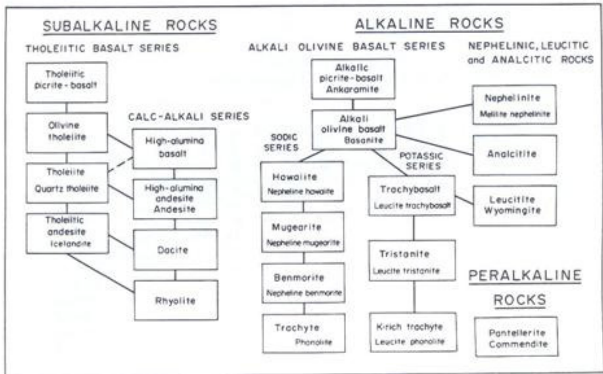
Figure 4-5 General classification scheme for the common volcanic rocks (after Irvine and Baragar, 1971). Lines joining boxes link commonly associated rocks. The small print within the boxes refers to variants of the main rock. (Published with permission of Canadian J. Earth Sci.)
