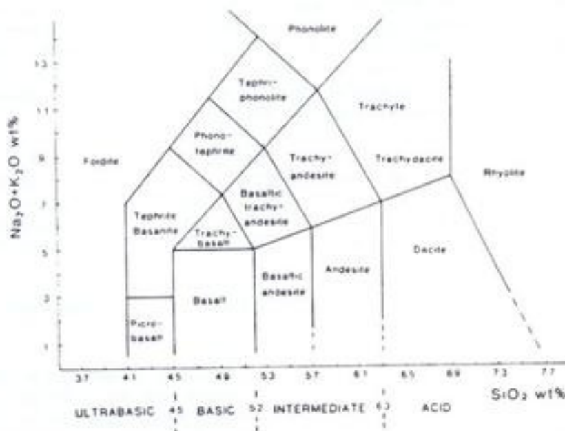
Figure 4-4 Compositional fields of volcanic rocks in terms of total alkalis and silica. (after Le Bas, et al., 1986; published with permission of Oxford University Press)
