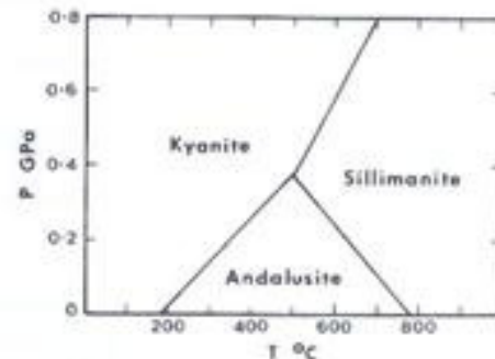
Phase relations among the \text{Al}_2\text{SiO}_5 polymorphs (Holdaway, 1971).
