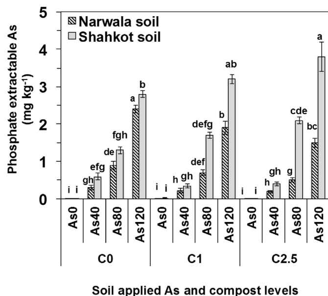
Fig. 2. Phosphate extractable (bioavailable) As concentration in the post-experimental Narwala and Shahkot soils under the influence of arsenic (As; 0, 40, 80, 120 mg kg -1 ) and compost (C; 0, 1, 2.5%) treatments. Data are presented as mean ± standard error of three replicates. Means followed by the same letter are not significantly different (Duncan's multiple-range test, p < 0.05).
