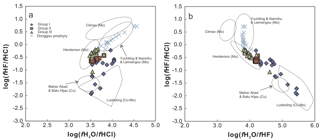
(Siahcheshm et al., 2012) in eastern Iran, and Batu Hijau (Idrus et al., 2007) in Indonesia and in the porphyry Cu-Mo-related plutons in the Luoboling (Li and Jiang, 2015) in south China based on the equations of Munoz (1992), and temperatures established from mineral or mineral pair geothermometry, e.g., 720 °C for Climax, 612–768 °C for Henderson, 758 °C for Maher Abad, 764 °C for Batu Hijau and 750 °C for Luoboling.
