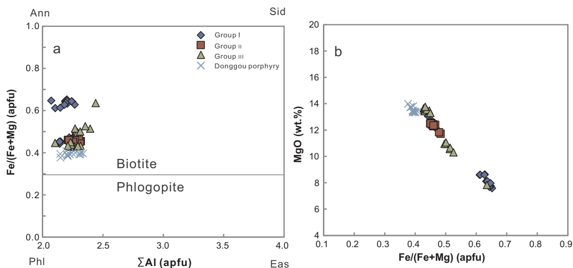
Fig. 4. Chemical compositional diagrams of biotite from the Taishanmiao batholith and Donggou porphyry. (a) \text{Fe}/(\text{Fe} + \text{Mg}) - \Sigma\text{Al} (apfu) (apfu = atoms per formula unit) diagram after Rieder et al. (1998), (b) diagram of \text{MgO} (wt%) vs. \text{Fe}/(\text{Fe} + \text{Mg}) (apfu).
