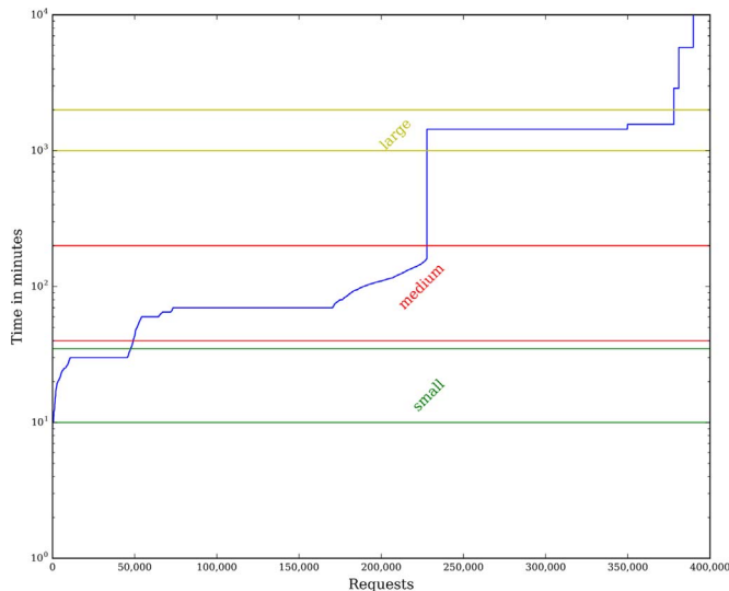
Fig. 5. Requested time window distribution – the figure represents a sample of real users' requests submitted to fdsnws-dataselect. The highlighted regions show the most popular time window lengths.
