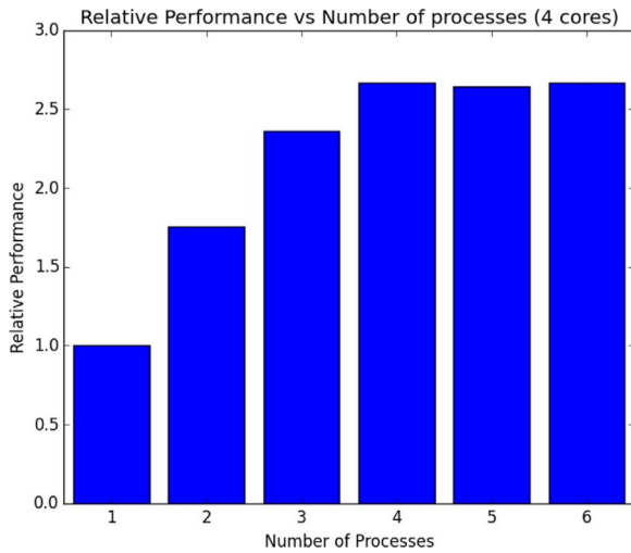
Fig. 4. The figure illustrates the behaviour of the WFCatalog ingestion process. The relative performance RelPerf = \frac{T_{1proc} * N_{proc}}{T_{Nproc}} is measured in terms of time.
