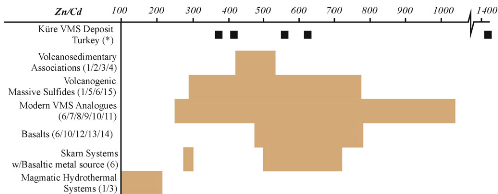
Fig. 8. Zn/Cd distributions of sphalerites from Küre VMS Deposit (*) with the data from different ore-forming systems and source rocks. Reference data are: (1) Xu, 1998; (2) Jonasson and Sangster, 1978; (3) Xuexin, 1984; (4) Brill, 1989; (5) Zaw and Large, 1996; (6) Gottesman and Kampe, 2007; (7) Goodfellow and Blaise, 1988; (8) Goodfellow and Franklin, 1993; (9) Hannington and Scott, 1988; (10) Bischoff et al., 1983; (11) Fouquet et al., 1993; (12) Turekian and Wedepohl, 1961; (13) Vinogradov, 1962; (14) Kay and Hubbard, 1978, (15) Herzig, 1988. Filled squares represent sphalerite data from massive ore of Küre deposit. Zn/Cd interval scheme adapted and modified from Gottesman and Kampe (2007).
