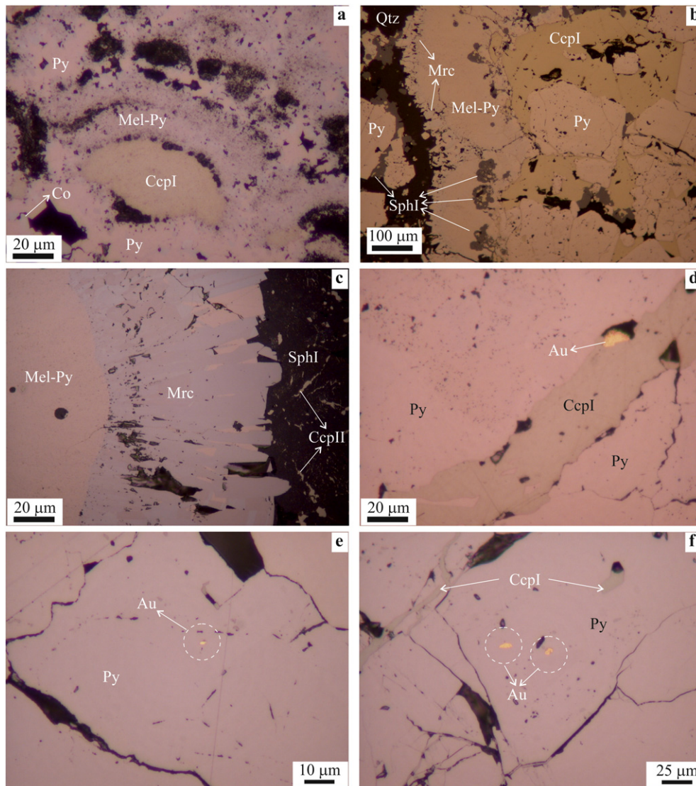
Fig. 7. Reflected-light images of the ore minerals from massive sulfide mineralization. (a) Cobaltite (Co)-pyrite (Py) intergrowths is being replaced by chalcopyrite-I (Ccpl) that is further replaced by melnicovite pyrite (Mel-Py). (b) Pyrite (Py) being replaced by chalcopyrite-I (Ccpl) and sphalerite-I (SphI). Chalcopyrite is further replaced by melnicovite pyrite (Mel-Py) and marcasite (Mrc). (c) Replacement of melnicovite pyrite (Mel-Py) by marcasite (Mrc). Marcasite is followed by sphalerite-I (SphI) that include chalcopyrite-II (CcplII) exsolution lamella. (d) Native gold (Au) at the boundary of pyrite (Py) and chalcopyrite-I (Ccpl). (e) and (f) Native gold (Au) as minute inclusions in pyrite. All images are in // nicols. Images (c) and (d) are in oil immersion.
