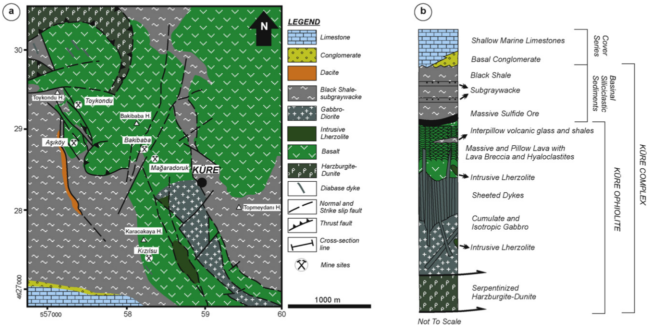
Fig. 2. (a) Geological map of the Küre VMS deposit and its surroundings (after Güner, 1980; Pehlivanoğlu, 1985; JICA and MMAJ, 1992; Çakır, 1995 and Çakır et al., 2006). (b) Generalized columnar section of the Küre ophiolite (modified after Ustaömer and Robertson, 1994).
