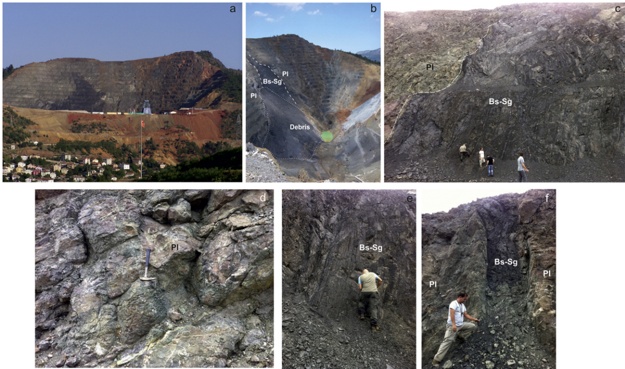
Fig. 3. (a) and (b) shows a general view of the Bakibaba Open-pit during the field studies in 2012, (b) and (c) steeply inclined contact of the Black shale–subgraywacke unit (Bs-Sg) and the pillow lavas (PI). (d) Pillow lava outcrop from the Bakibaba Open-pit. (e) Black shale–subgraywacke on bench face from the Bakibaba Open-pit. (f) Close-up view of the vertical segment of the black shale–subgraywacke–pillow lava contact.
