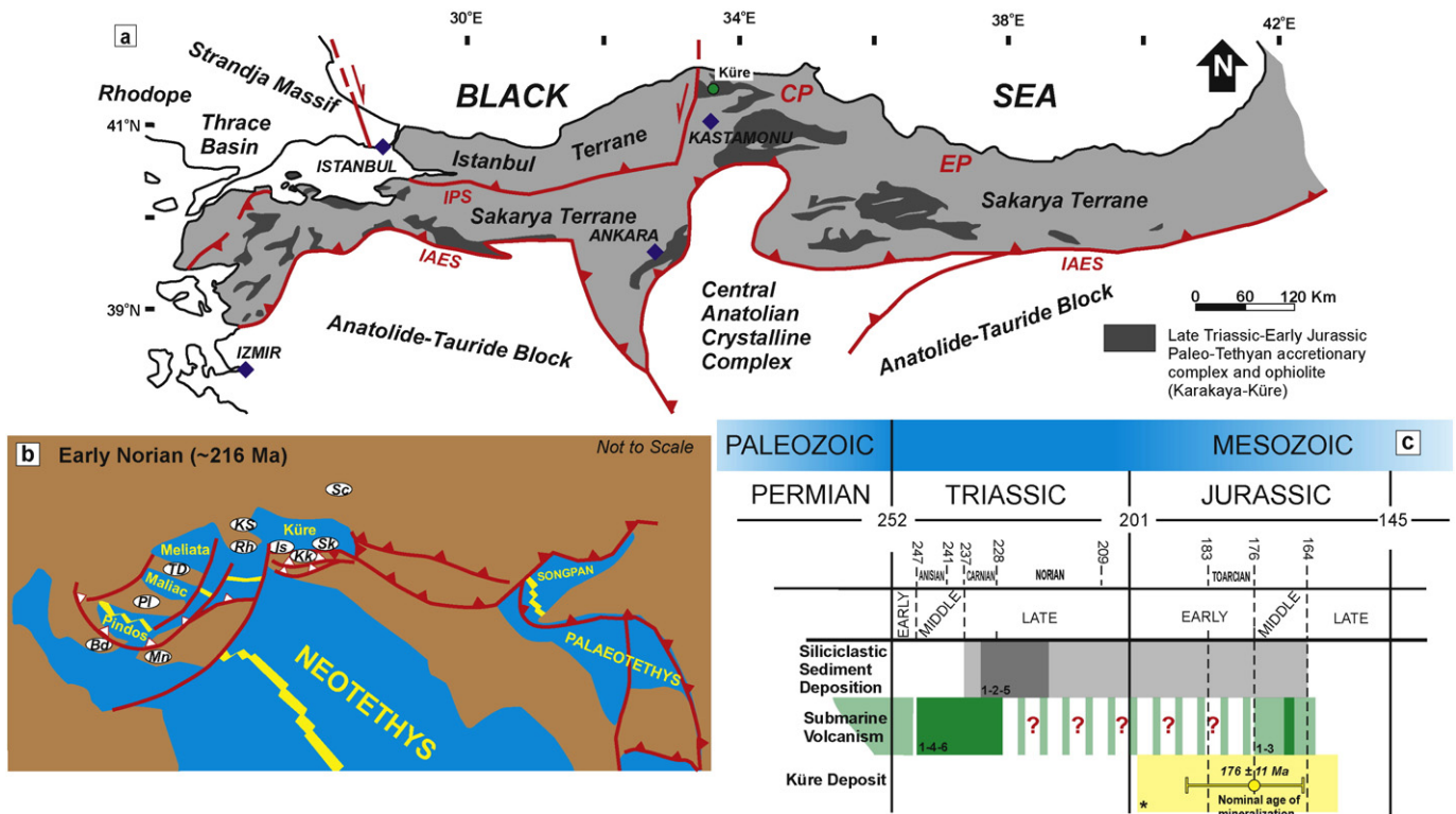
Fig. 12. (a) Tectonic map of northern Anatolia showing the distribution of the Late Triassic–Early Jurassic Paleo-Tethyan accretionary complex and ophiolite (Karakaya–Küre) (from Okay and Göncüoğlu, 2004). Light grey shaded region shows the Pontides. CP: Central Pontides, EP: Eastern Pontides, IAES: Izmir–Ankara–Erzincan Suture, IPS: Intra-Pontide Suture. (b) Schematic cartoon depicting the western Tethyan realm during Early Norian (from Stampfli et al., 2002). (b) Beydağlar; (Is) Istanbul; (Kk) Karakaya forearc; (KS) Kotel–Stranja rift; (Mn) Menderes; (Pl) Pelagonian; (Rh) Rhodope; (Sc) Scythian platform; (Sk) Sakarya; (TD) Trans-Danubian. (c) Summary of the Geological history of the volcano-sedimentary associations of Küre Complex and the Küre VMS Deposit. Reference data are from: (1) Kozur et al. (2000); (2) Aydın et al. (1995); (3) Terzioğlu et al. (2000); (4) Ustaömer and Robertson (1995); (5) Alişan et al. (1992); (6) Çakır (1995); (*) This study.
