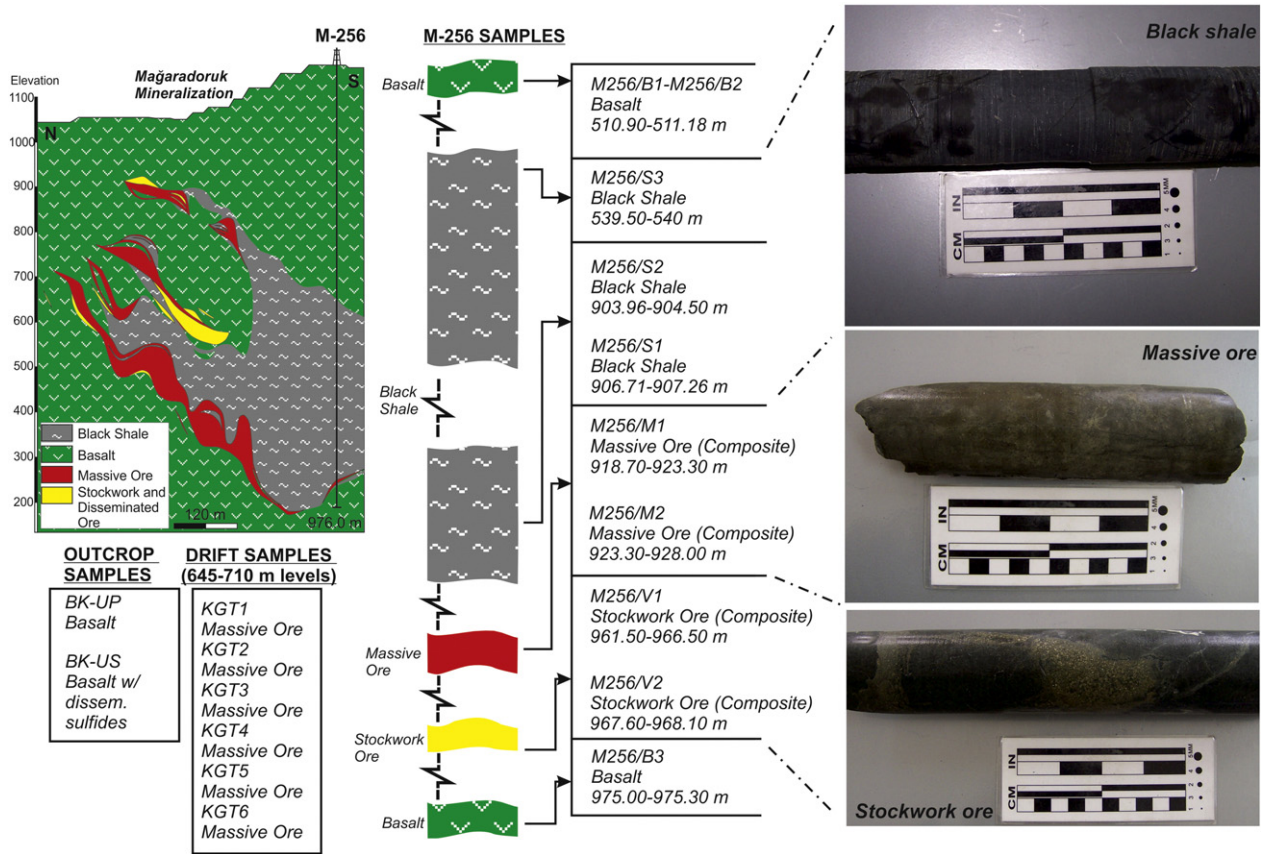
Fig. 5. A schematic summary of the sample depths, types, and lithologies. N–S oriented cross-section of the Mağaradoruk mineralization is from Altun et al. (2015).
