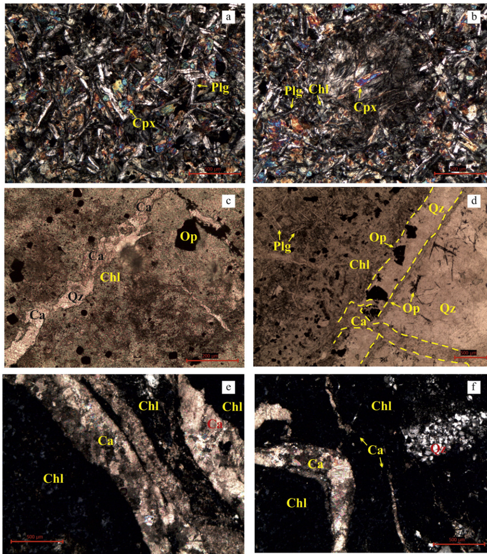
Fig. 4. Photomicrographs of the (a and b) fresh (unaltered) and (c, d, e, f) altered (heavily chloritized) basaltic pillow lavas. Note the overprinting quartz and calcite stockwork veinlets in (c, d, e and f). Cpx: clinopyroxene, Plg: plagioclase, Chl: chlorite, Qz: quartz, Ca: calcite, Op: opaque phases. Photomicrographs (a, b, e and f) are in (+), (c, d) are in (//) nicols.
