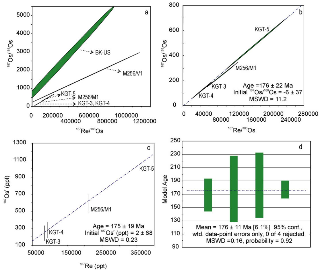
Fig. 11. (a) ^{187}\text{Re} - ^{188}\text{Os} vs. ^{187}\text{Os} - ^{188}\text{Os} plot for all of the six Küre VMS pyrite concentrates. (b) ^{187}\text{Re} - ^{188}\text{Os} vs. ^{187}\text{Os} - ^{188}\text{Os} isochron for four of the pyrite concentrates. (c) ^{187}\text{Re} - ^{187}\text{Os}^f isochron for the same set of pyrite concentrates. (d) Weighted average of the model ages plotted for the Küre VMS deposit samples. The data-point error ellipses in (a), (b) and (c), and the box heights in (d) donate 2SE.
