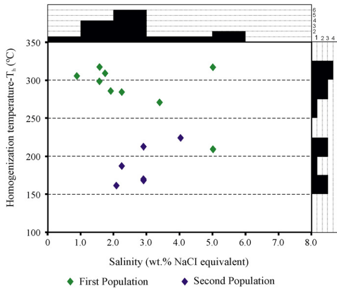
Fig. 10. A diagram-histogram composite of homogenization temperatures ( T_h ) and the fluid salinities obtained by the microthermometric measurements from the quartz of the stockwork ore of the Küre VMS deposit.
