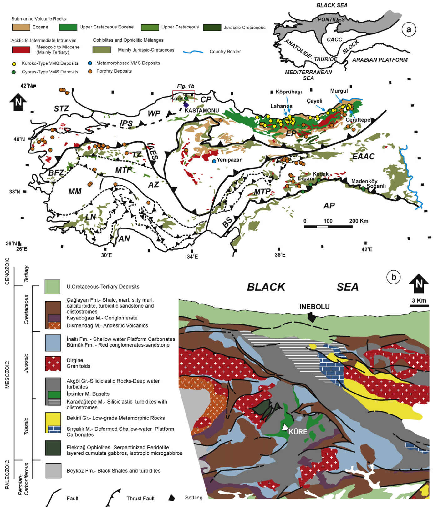
Fig. 1. (a) Distribution of submarine volcanic, ophiolitic and acidic to intermediate intrusive host rock assemblages and related VMS and Porphyry Deposits of Turkey, with respect to the Palaeo-tectonic units (after Yiğit, 2009). STZ: Strandja Zone, WP: Western Pontides, CP: Central Pontides, EP: Eastern Pontides, BFZ: Bornova Flysch Zone, TZ Tavşanlı Zone, MM: Menderes Massif, MTP: Menderes-Taurus Platform, AZ: Afyon Zone; CACC: Central Anatolian Crystalline Complex, EAAC: Eastern Anatolian Accretionary Complex, IAES: Izmir-Ankara-Erzincan Suture, BS: Bitlis Suture, IPS: Intra-Pontide Suture. (b) Regional Geological Map of the Küre and surroundings (modified after Aydın et al., 1995; Kozur et al., 2000). Fm: formation, M: member, Gr: Group.
