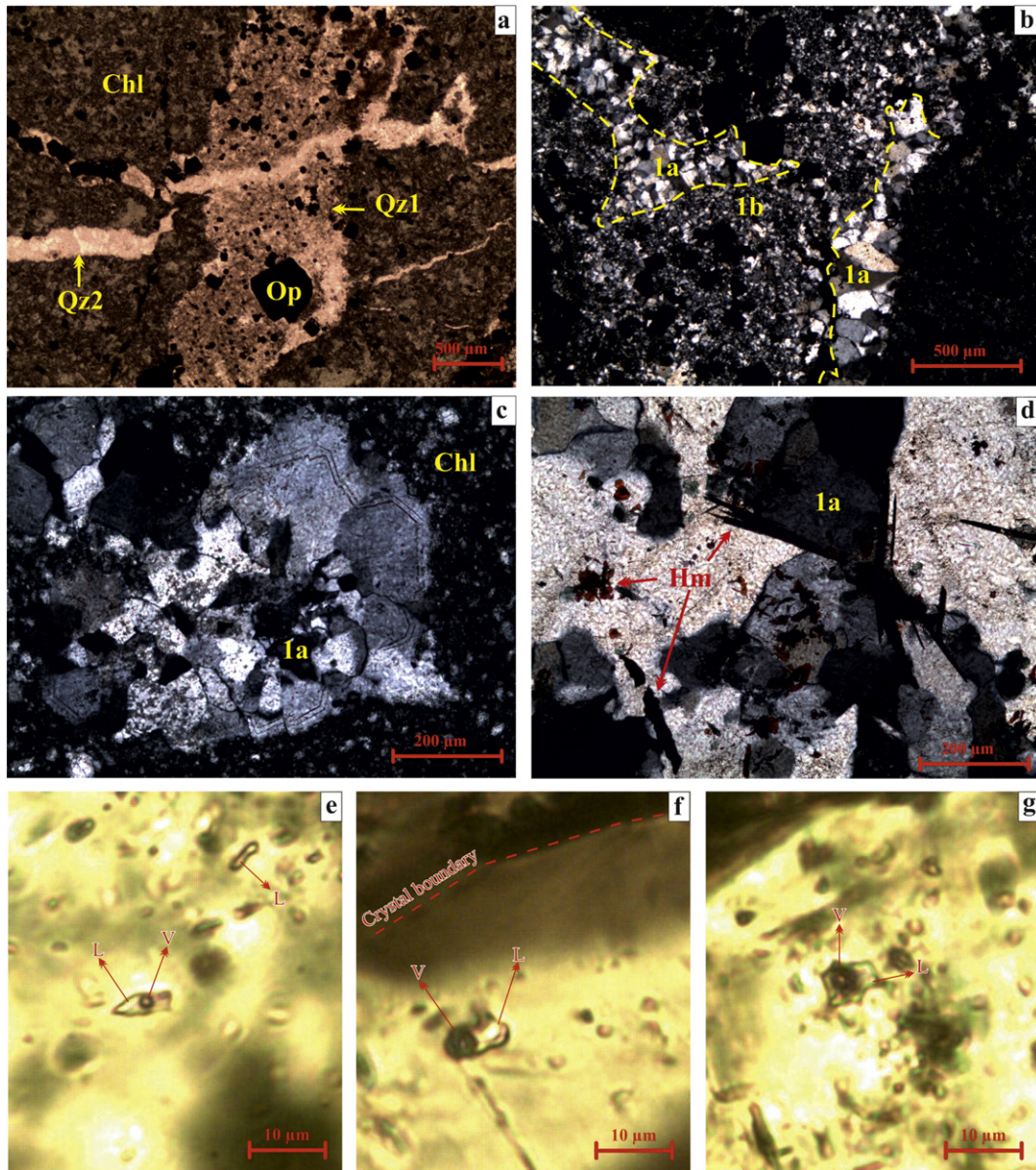
Fig. 9. Photomicrographs of the veinlets and the hosted fluid inclusions in the stockwork zone of the Küre massive sulfide mineralization. (a) to (d) show early and late stage quartz veinlets (Qz1 and Qz2, respectively) and, (1a) and (1b) represents early and late stage in the (Qz1). (e), (f) and (g) show samples of two phase fluid inclusions from the quartz veinlets of the stockwork ore, (L and V denotes liquid and vapor phases respectively).
